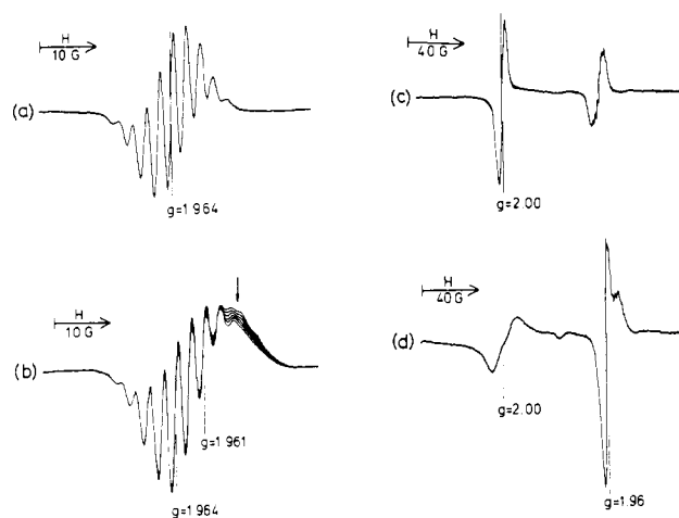
Figure 8. ESR spectra for the range of I = 0 during the electrochemical reduction of Mo(O)(TPP)(MeO) (2.0 × 10 -3 M) in dichloromethane containing 0.10 M TBAP at room temperature: (a) before electrolysis; (b) reoxidation after complete electrolysis at -0.8 V vs. SCE, followed by reduction at -0.5 V vs. SCE (the region of signal decay is shown by an arrow); (c) reduction at -1.3 V vs. SCE (the signal due to 1 still remains for this reduction time); (d) reduction at -2.0 V vs. SCE.
