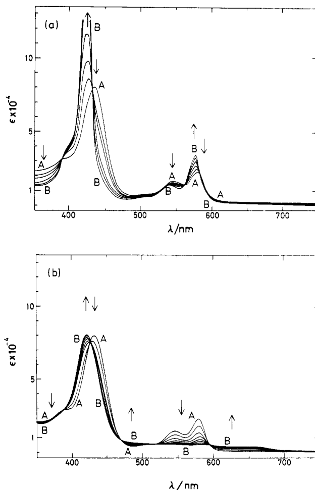
Figure 3. Electrochemical reduction (at -1.0 V vs. SCE) and oxidation (at 1.0 V vs. SCE) of Mo(O)(MEC) ( 1.5 \times 10^{-5} M) in dichloromethane containing 5.0 \times 10^{-2} M TBAP at 15 °C: (a) A, Mo V (O)(MEC); B, one-electron-reduced species; (b) A, Mo V (O)(MEC); B, one-electron-oxidized species. Trends of spectral changes with time are shown by arrows.
