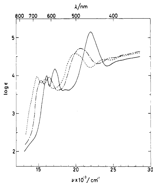
Figure 4. Electronic spectra of Mo V porphyrins in dichloromethane at 25.0 ± 0.2 °C: —, Mo(O)(TPP)(MeO); ---, Mo(O)(TPP)(AcO); - · - ·, Mo(O)(TPP)Cl.
